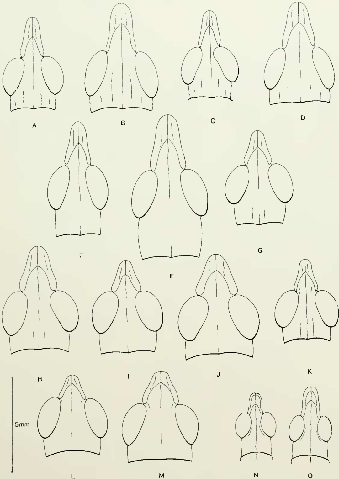
Figure 1. Dorsal view of heads of Ichthiacris spp. A, B, I. (I.) rehni , ♂, ♀; C, I. (I.) spinifera , ♂, holotype; D, I. (I.) spinifera , ♀ allotype; E, F, I. (Atyphacris) elongata , ♂, ♀; G, H, I. (A.) costulata , ♂, ♀; I, J, I. (A.) californica , ♂, ♀; K, I. (A.) celata , ♂; L, M, I. (A.) aptera , ♂, holotype; O, I. (I.) parva , ♀; N, I. (I.) parva , ♂, ♀ (last-instar juv.).
